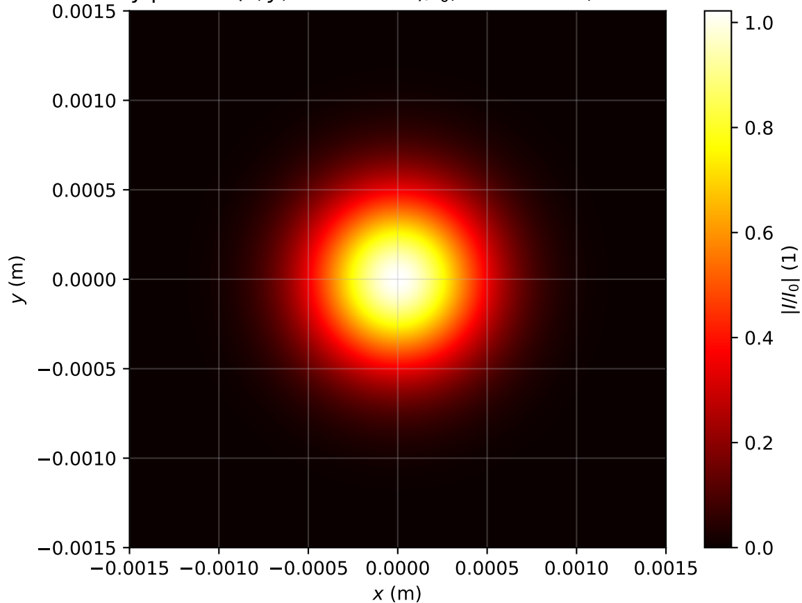
Intensity profile I(x, y, z = 0.318m)/I_0 , P_{in}=0.5P_{cr} , artificial time
